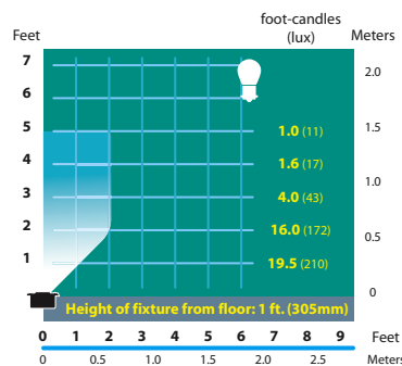
SL-02-3L Half Spread Photometrics
