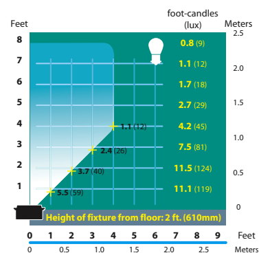
SL-31 Half Spread Photometrics
