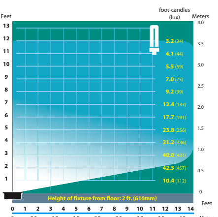
SL-08-FL-9 Half Spread Photometrics (9w)
