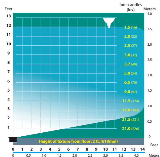
SL-17-AL-MR16 Half Spread Photometrics (20w)
