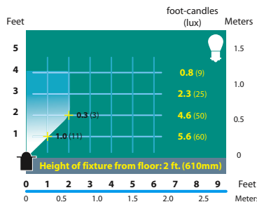
SL-24 Half Spread Photometrics
