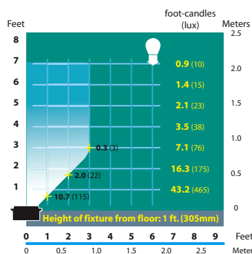
SL-31 Half Spread Photometrics
