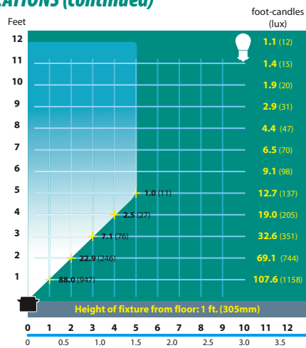
SL-30 Half Spread Photometrics
