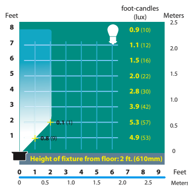
SL-17-AL Half Spread Photometrics
