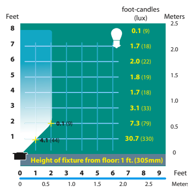
SL-02 Half Spread Photometrics
