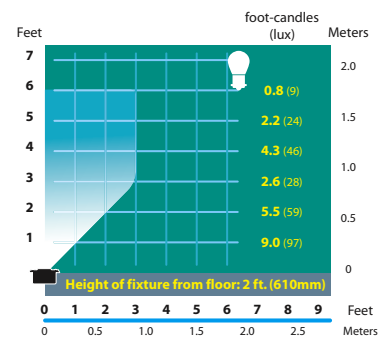
SL-02-3L Half Spread Photometrics
