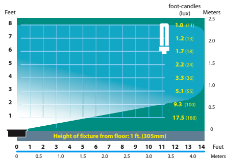
SL-08-AL-FL-5 Half Spread Photometrics (5w)
