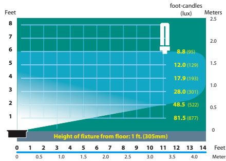
SL-08-AL-FL-7 Half Spread Photometrics (7w)
