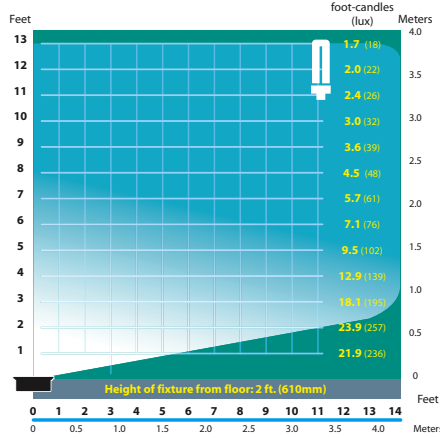
SL-08-AL-FL-7 Half Spread Photometrics (7w)
