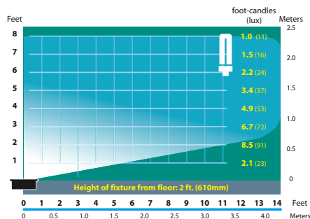
SL-08-FL-5 Half Spread Photometrics (5w)
