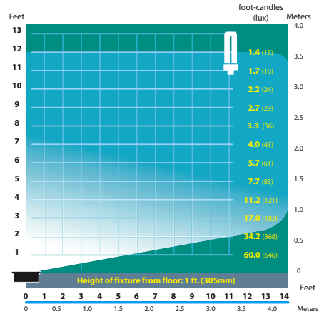
SL-08-AL-FL-9 Half Spread Photometrics (9w)
