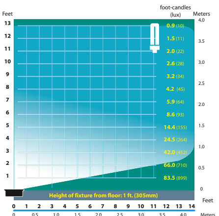
SL-08-FL-7 Half Spread Photometrics (7w)
