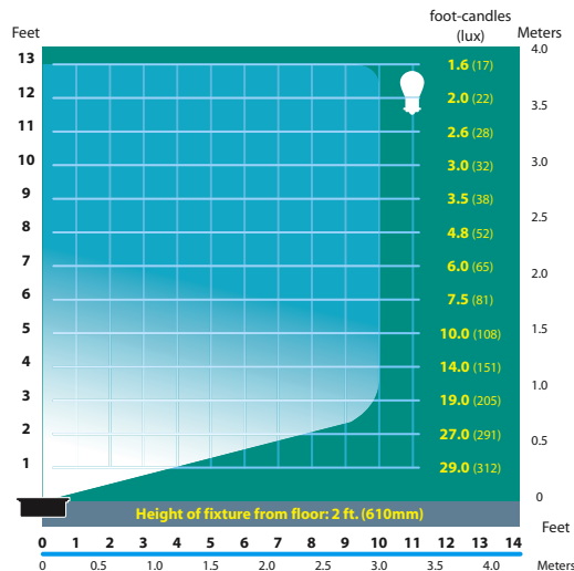
SL-04-AL Half Spread Photometrics
