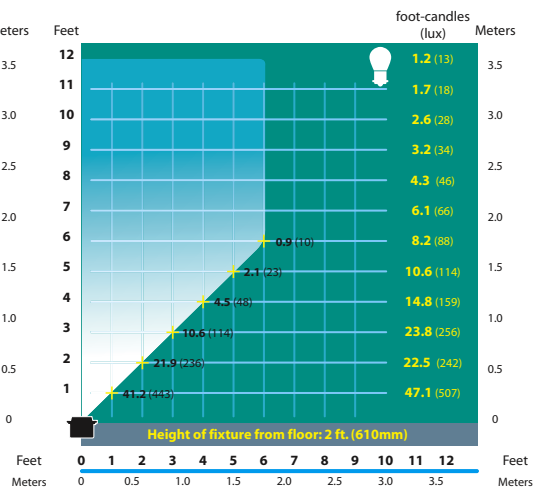
SL-30 Half Spread Photometrics
