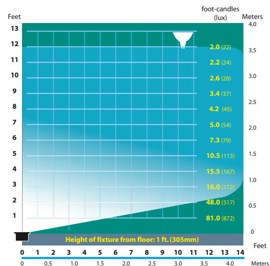
SL-17-AL-MR16 Half Spread Photometrics (20w)
