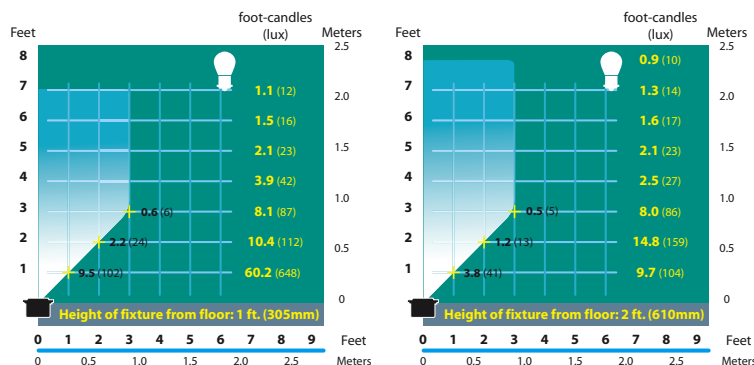
SL-17 Half Spread Photometrics
